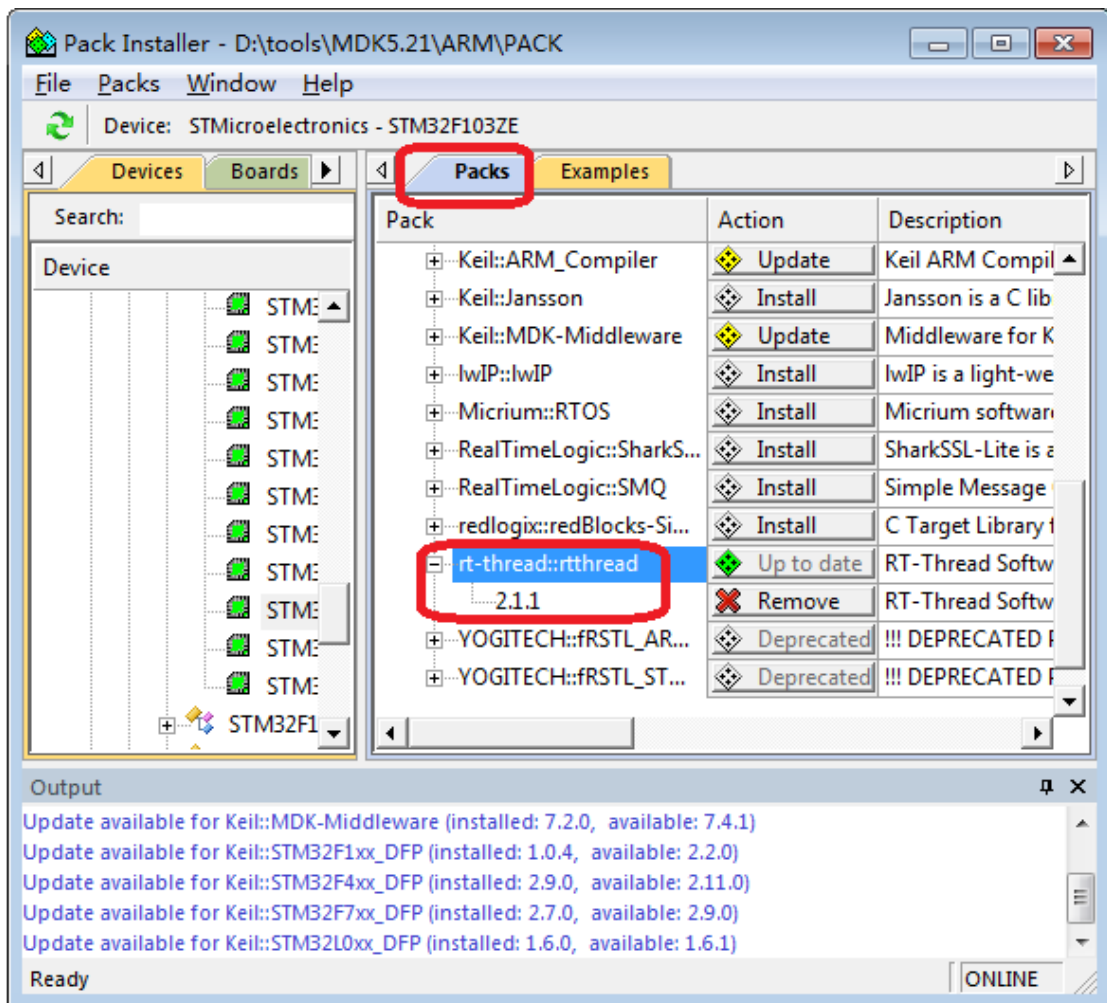
图 2: RT-ThreadPack 下载
