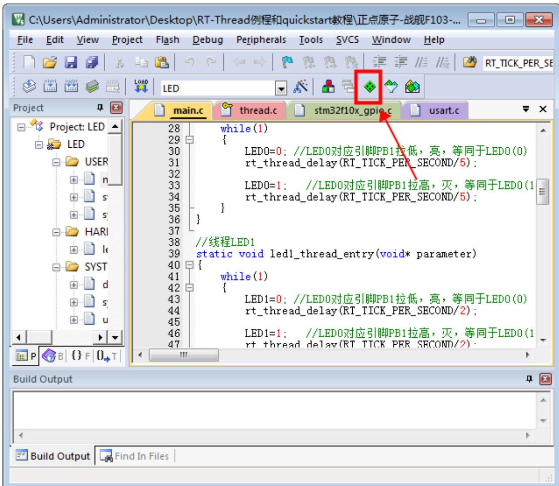
图 4: ManageRun-Time Environment
